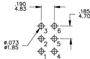
P.C. MOUNTING
