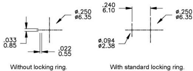
PANEL MOUNTING
