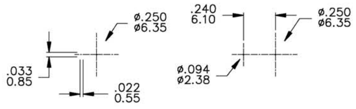
PANEL MOUNTING
