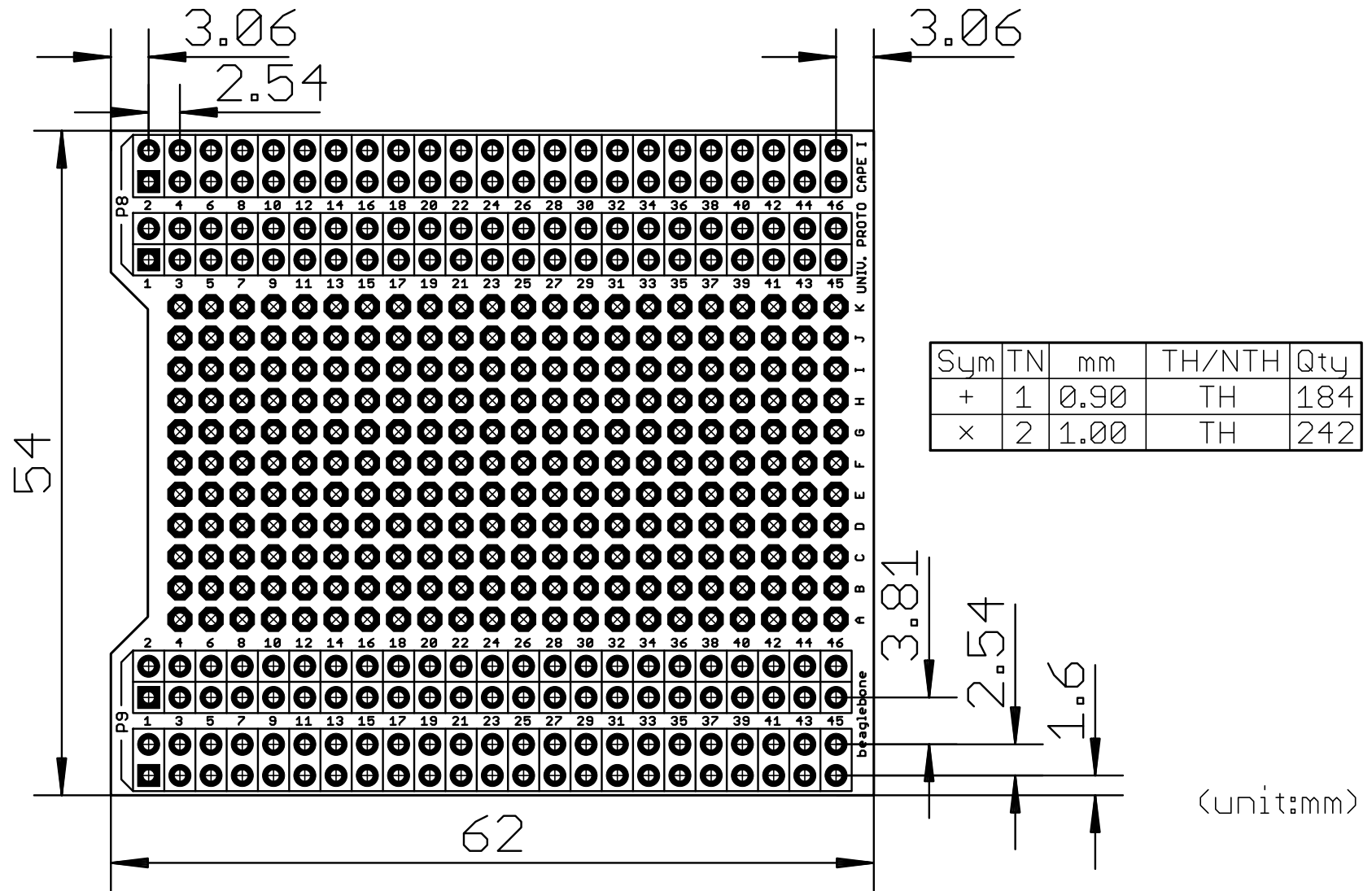
BEAGLEBONE-UNIVERSAL-CAPE1
