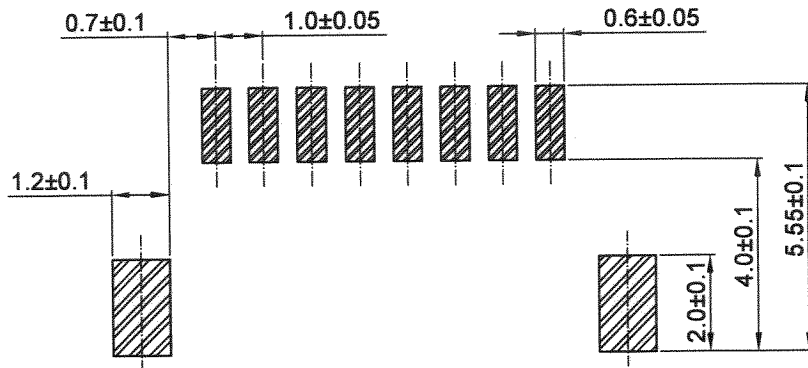
RECOMMENDED P.C.BOARD PATTERN DIM.
