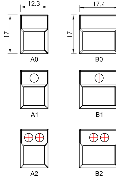
CONTACT CONFIGURATION
