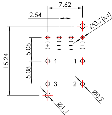
P.C.B. MOUNTING HOLES
