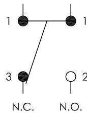
CONTACT CONFIGURATION
