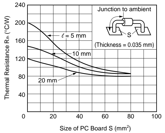
Fig. 8 Rth-S CHARACTERISTIC
