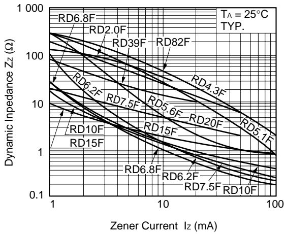
Fig. 7 Zz-Iz CHARACTERISTIC
